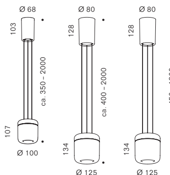
CAVITY Suspension S, L CAVITY Suspension Adjustable L
