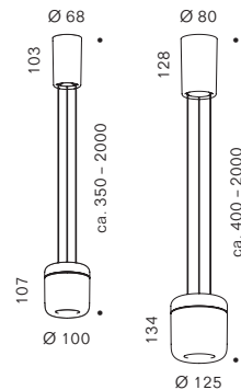
CAVITY Suspension S, L
