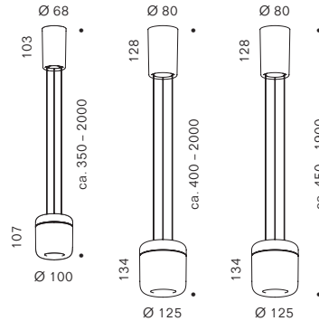
CAVITY Suspension S, L CAVITY Suspension Adjustable L
